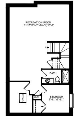
1 BEDROOM 'LEGAL SUITE' 727 SQ FT
