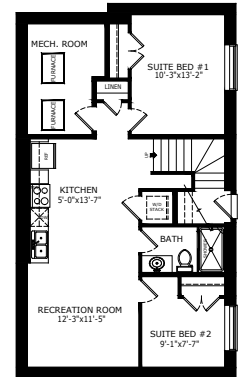
2 BEDROOM 'LEGAL SUITE' 727 SQ FT
