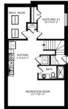
2 BEDROOM 'LEGAL SUITE' 727 SQ FT
