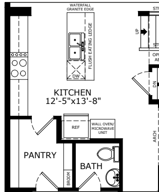
OPTIONAL EXECUTIVE KITCHEN
